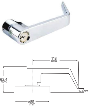
Lever (L)
