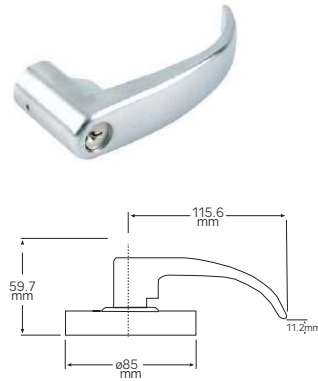
Lever (R)
