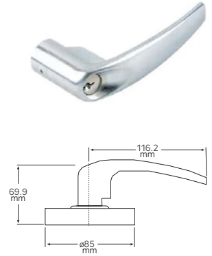
Lever (S)
