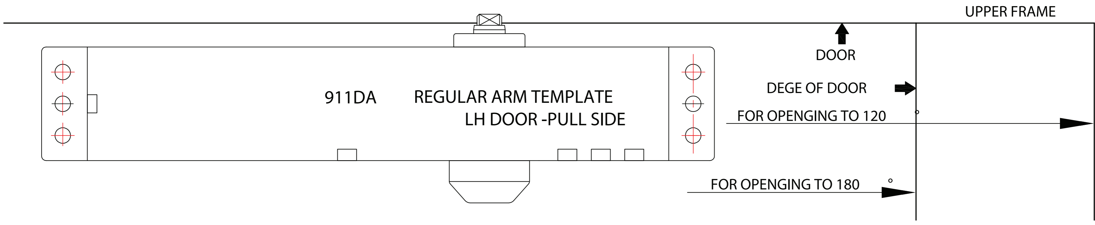
REGULAR ARM APPLICATION TEMPLATE FOR A LEFT HAND DOOR PULL SIDE
