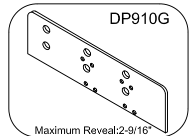
Top Jamb Drop Down Drop plate
