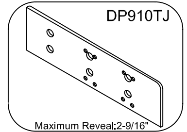
Top Jamb Center Mount Drop plate
